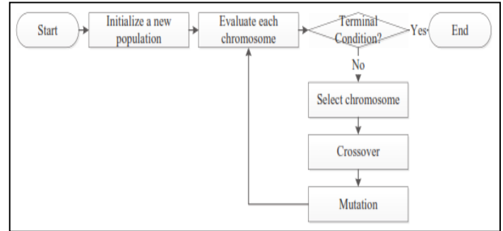
Figure: Genetic Algorithm process
