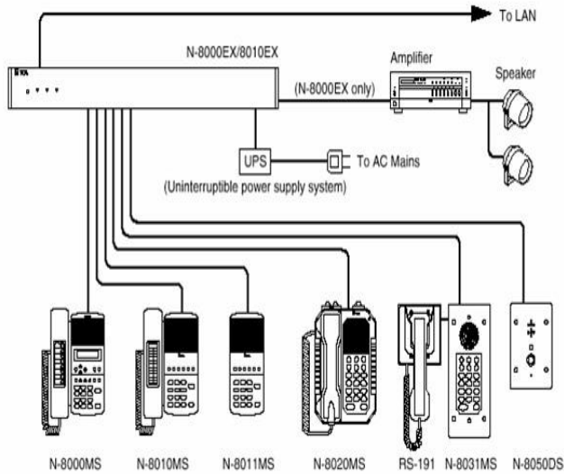
Fig 1. Intercom Connections
