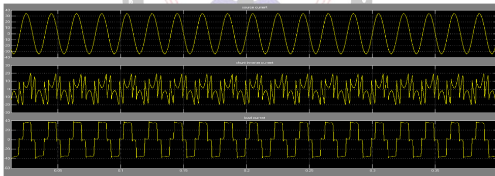
Fig5. Current harmonic compensation (a) Source current (b) Shunt inverter current (c) Load current
