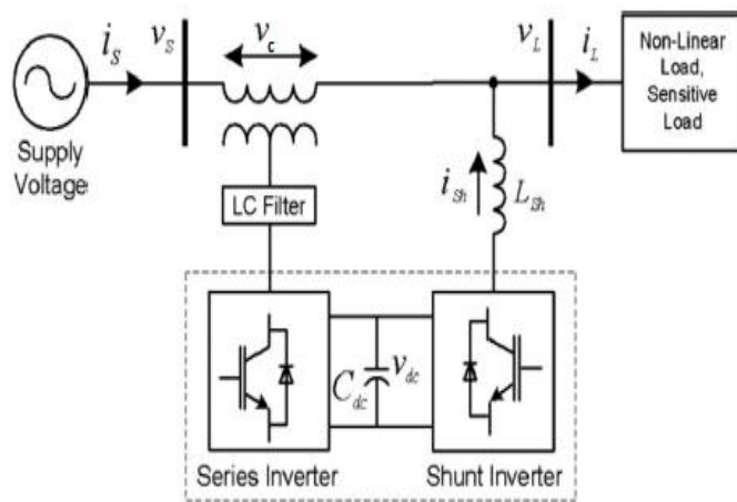
Fig1. General block diagram of UPQC
