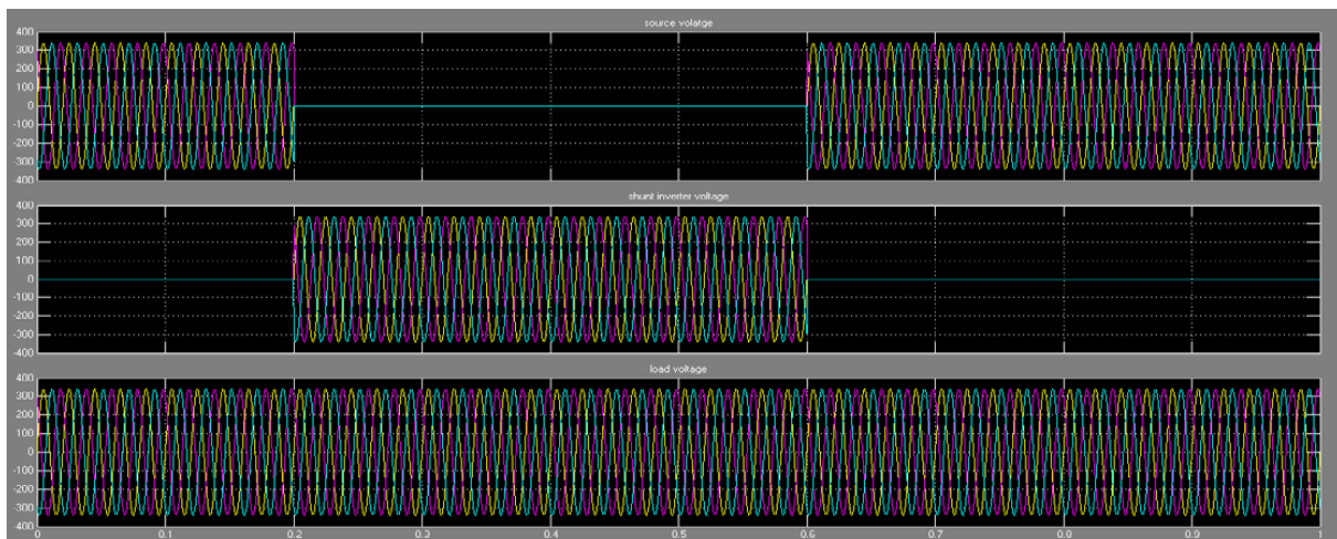
fig9. Voltage interruption (forward flow mode) (a) Source voltage (b) shunt inverter voltage (c) load voltage
