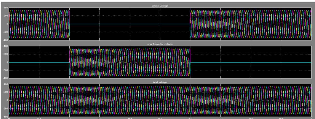
fig12. Voltage interruption (reverse flow mode) (a) Source voltage (b) Shunt inverter voltage (c) Load voltage
