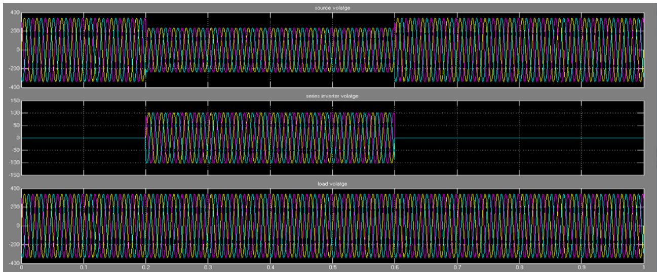
Fig11. Balanced voltage sag compensation. (a) Source voltage (b) Series inverter voltage (c) Load voltage
