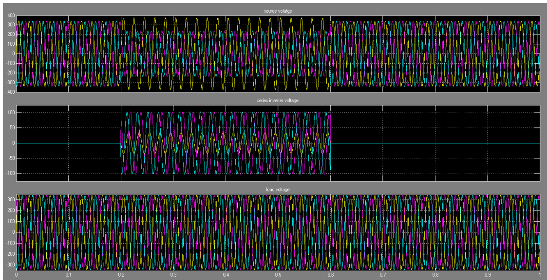
fig7. Voltage sag compensation (unbalanced voltage sag) (a) Source voltage (b) Series inverter voltage (c) Load voltage
