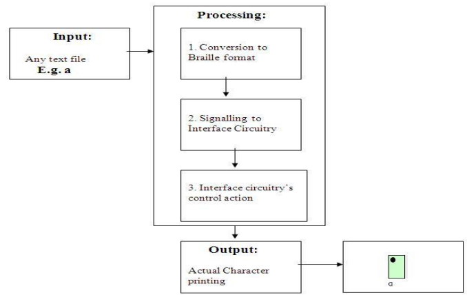
Fig.2 System Overview
