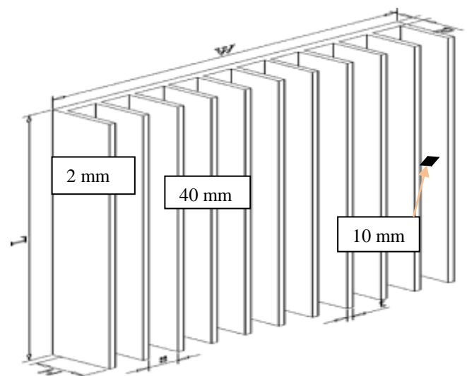
Figure01: Protruded rectangular fin
