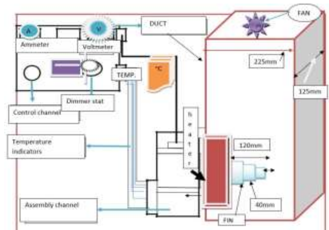
Figure 04:Block diagram of experimental setup
