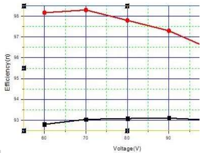
Figure 08: Graph of voltage Vs Efficiency in natural convection
