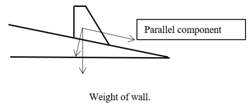
1 Figure Concept of resistance by sliding on inclined plane.
