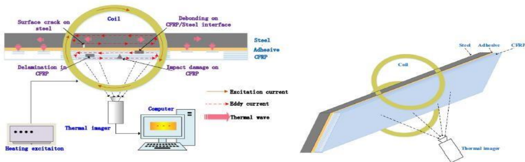
Fig. 1. Schematic of the proposed method for defects detection in CFRP
