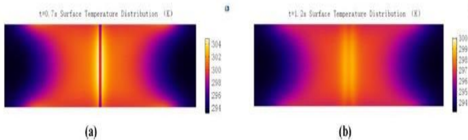
Fig. 12. The temperature distributions of different surfaces of CFRP strengthened steel structure with crack: (a) steel bonding surface; (b) CFRP surface.
