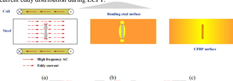
Fig. 3. Electromagnetic and thermal response of a CFRP-steel bonded structure with a crack in the steel bonding surface: (a) the electromagnetic response (b) the thermal response during the heating stage (c) the thermal response after heating.
