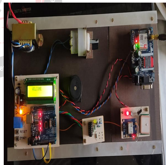
Fig-10: Prototype
