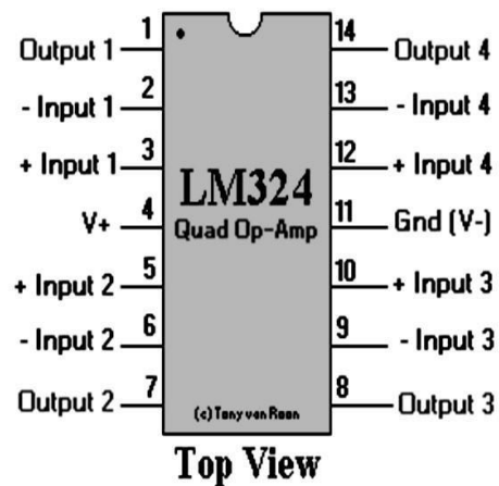
Fig-8: LM324 pin diagram
