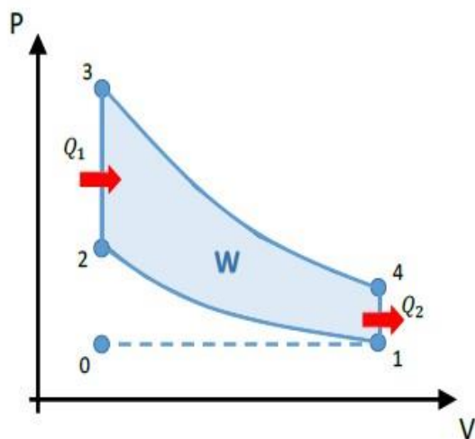
Figure: p/V diagram of the Otto cycle.
