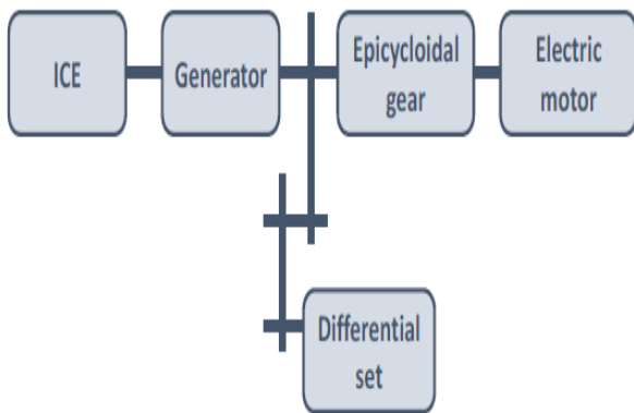
Schematic diagram of a typical hybrid transmission system
