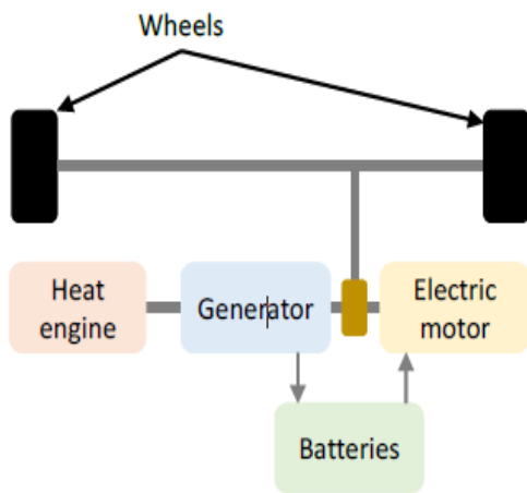
Typical architecture of an HEV with full-hybridization level
