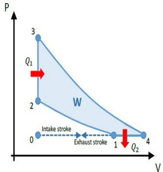
p/V diagram of the Atkinson cycle.
