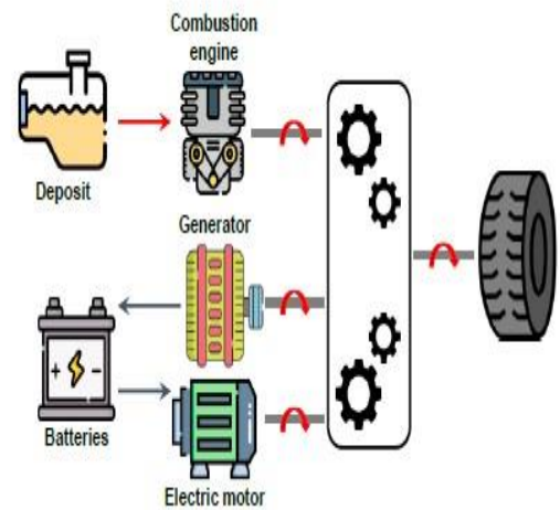
Mixed configuration of an HEV
