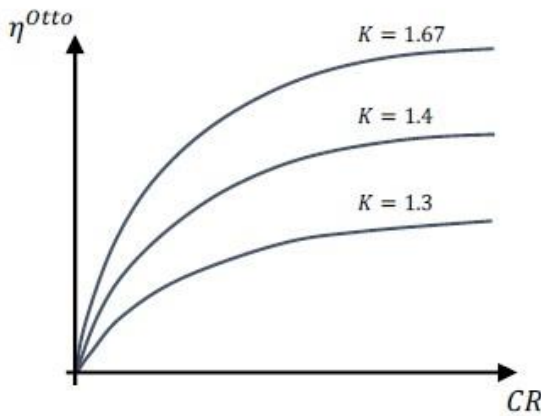
Thermal efficiency of the Otto cycle as function of the specific-heat and compression ratios
