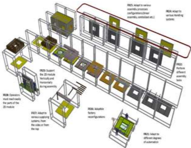
Figure 1. Sub-System 2: Robotic manufacturing system for building refurbishment, a scheme
