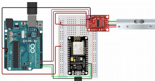
Figure 4. Circuit Diagram
