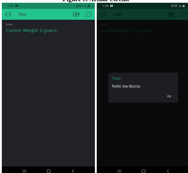
Figure 6. Mobile Application
