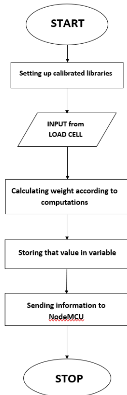
Figure 2. Algorithm for Arduino
