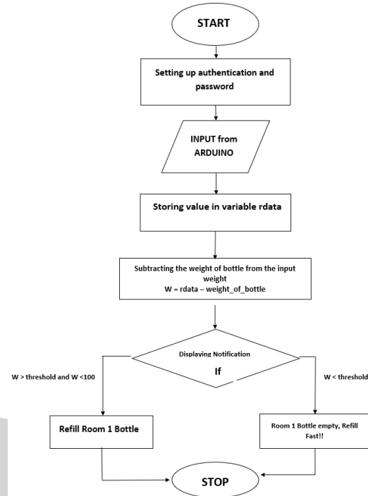
Figure 3. Algorithm for NodeMCU
